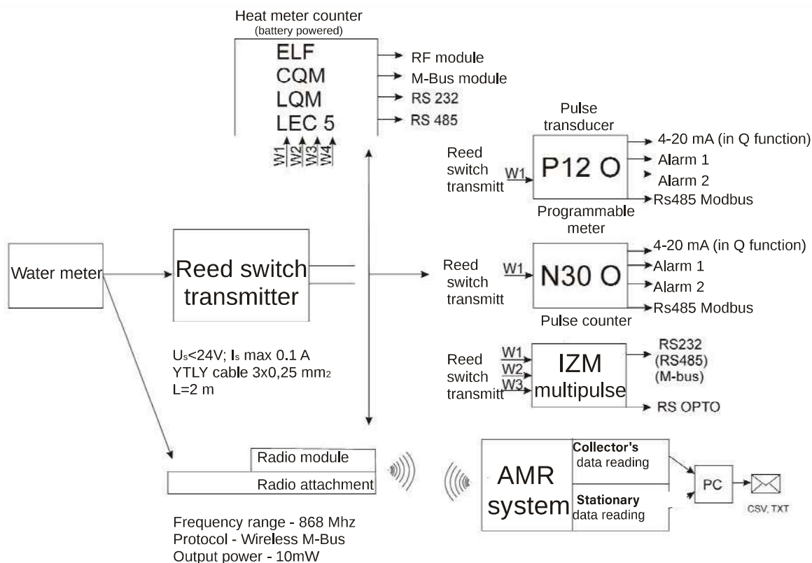
Fig. 5 Example connection scheme for remote transfer of readings
